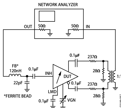
图57. 测试电路—频率响应(末端接LNA, R_s = 50 \Omega )
