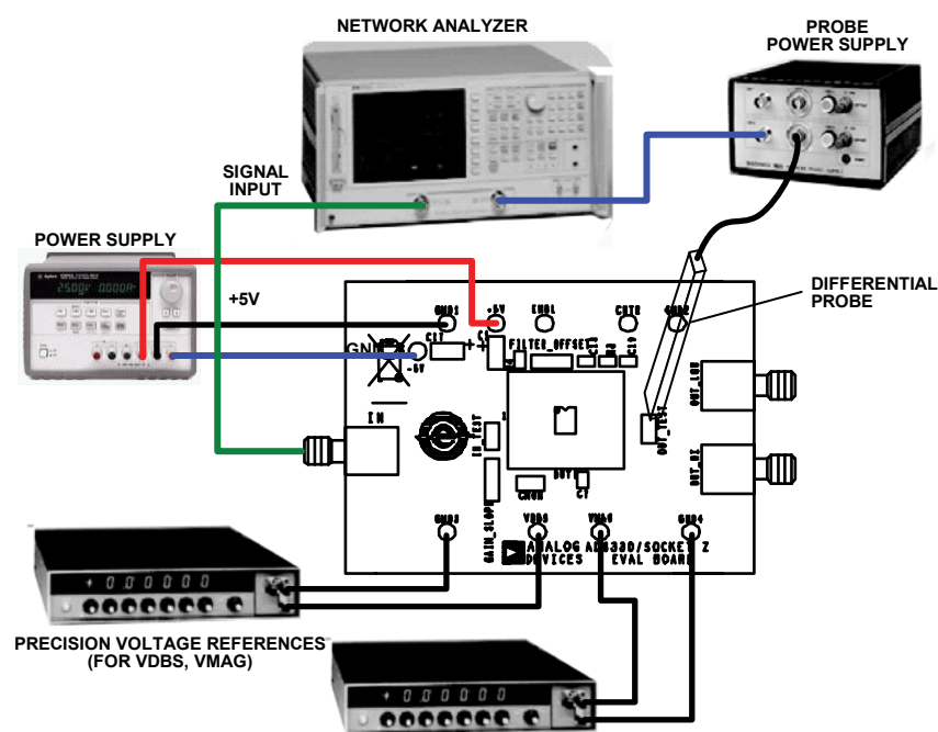
Figure 71. Typical Connections
