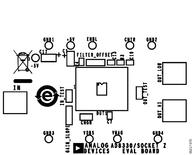
Figure 72. Component-Side Silkscreen
