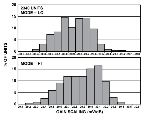
Figure 8. Gain Slope Histogram
