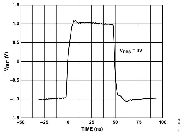
Figure 33. Full-Scale Transient Response, V_{DBS} = 0\text{V}
