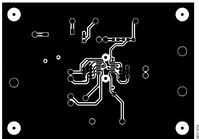
Figure 73. Component-Side Wiring
