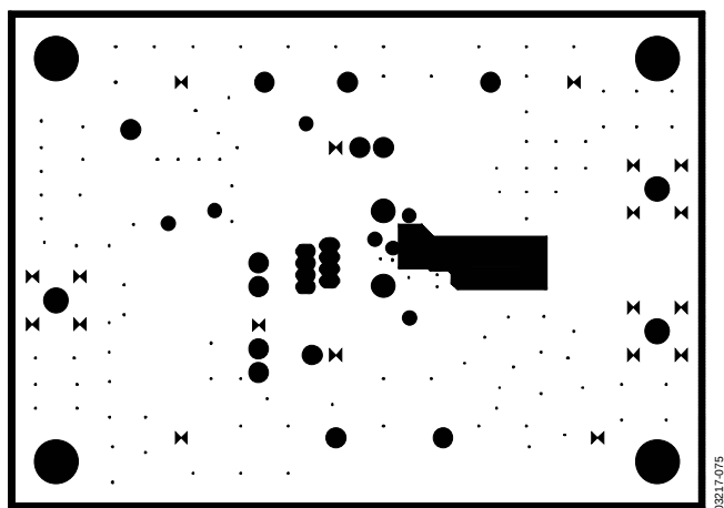
Figure 74. Ground Plane
