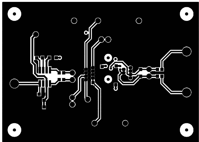
Figure 76. Wiring-Side Pattern
