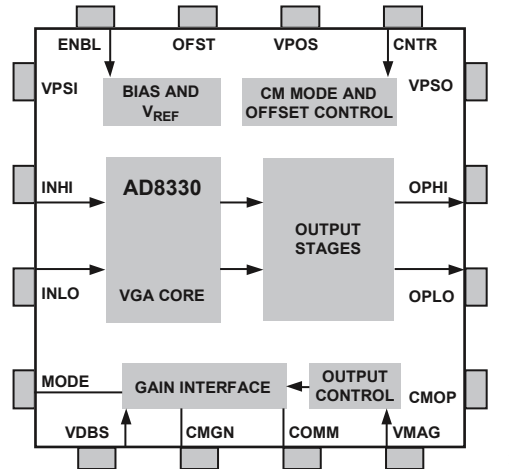
Figure 46. Block Schematic
