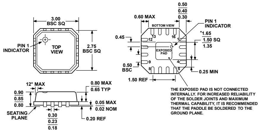
Figure 78. 16-Lead Lead Frame Chip Scale Package [LFCSP_VQ] 3 mm x 3 mm Body, Very Thin Quad (CP-16-3) Dimensions shown in millimeters
