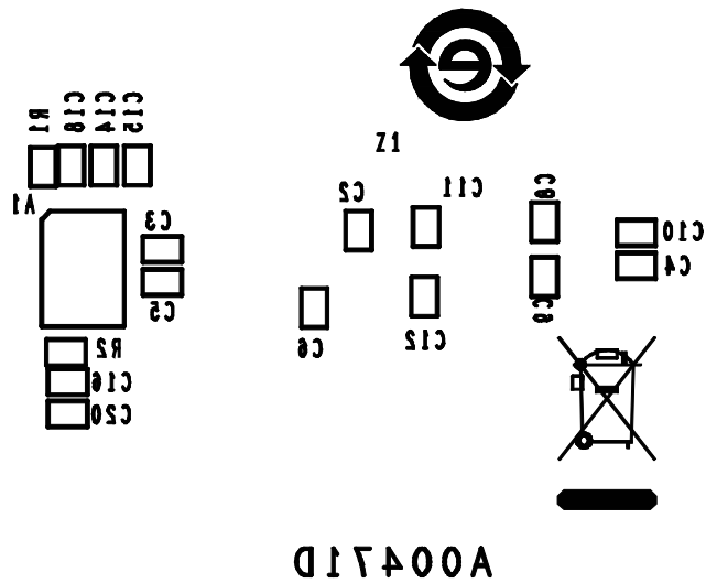
Figure 75. Wiring-Side Silkscreen
