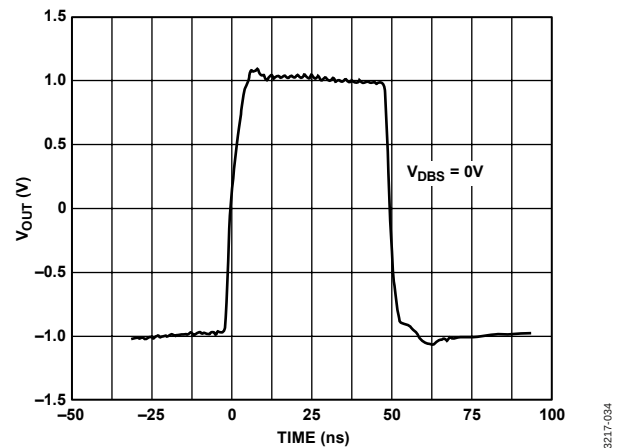
Figure 33. Full-Scale Transient Response, V_{DBS} = 0\text{V}
