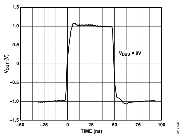
Figure 33. Full-Scale Transient Response, V_{DBS} = 0V
