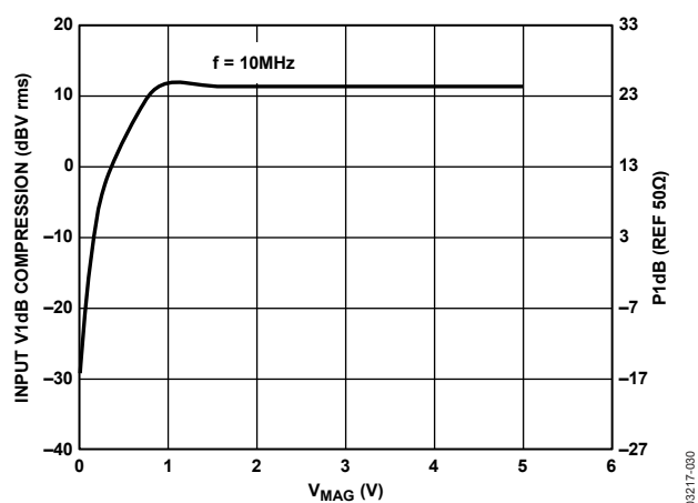
Figure 29. Output V1dB Compression vs. V_{MAG}
