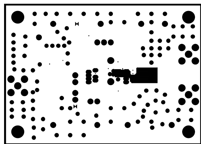
Figure 77. Inner Layer 2
