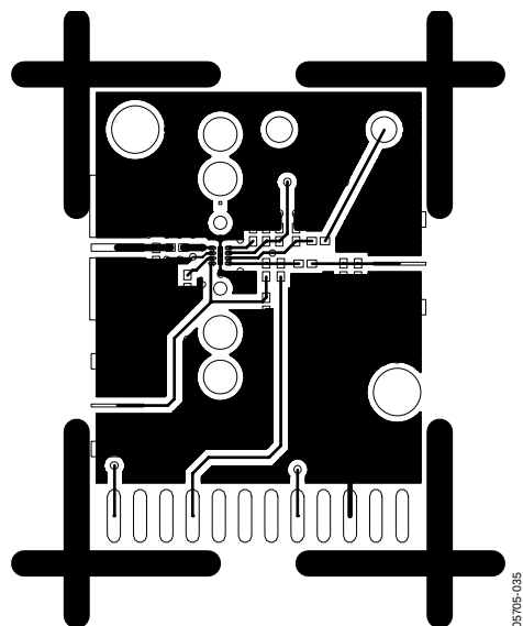
Figure 37. Component Side Layout
