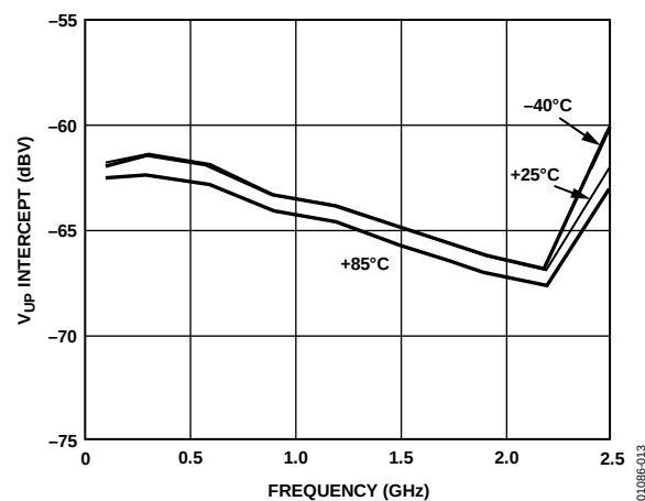
Figure 13. V_{UP} Intercept vs. Frequency; -40°C, +25°C, and +85°C
