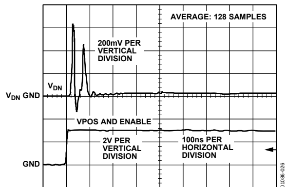
Figure 26. Power-On Response, V_{DN} Controller Mode with VSET Held Low
