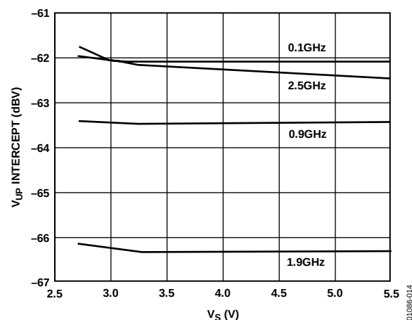
Figure 14. V_{UP} Intercept vs. Supply Voltage
