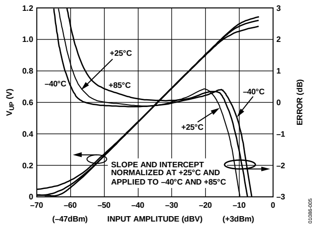
Figure 5. V_{UP} and Log Conformance vs. Input Amplitude at 0.1 GHz; -40°C, +25°C, and +85°C
