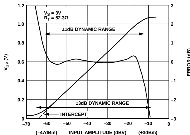
Figure 32. V UP and Log Conformance Error vs. Input Level at 900 MHz
