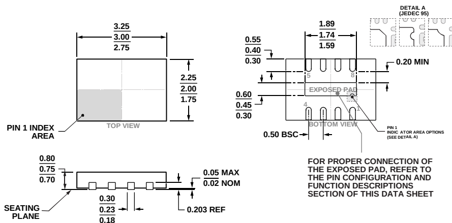
Figure 49. 8-Lead Lead Frame Chip Scale Package [LFCSP] 2 mm × 3 mm Body and 0.75 mm Package Height (CP-8-23)
