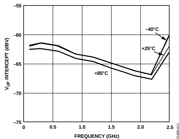
Figure 13. V_{UP} Intercept vs. Frequency; -40^{\circ}\text{C} , +25^{\circ}\text{C} , and +85^{\circ}\text{C}
