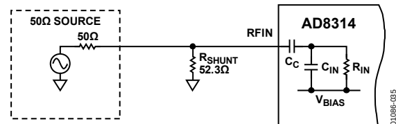
Figure 35. Broadband Resistive
