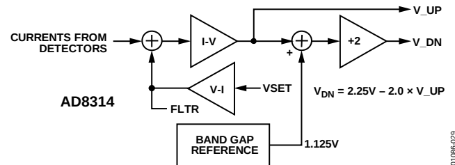
Figure 29. Output Interfaces
