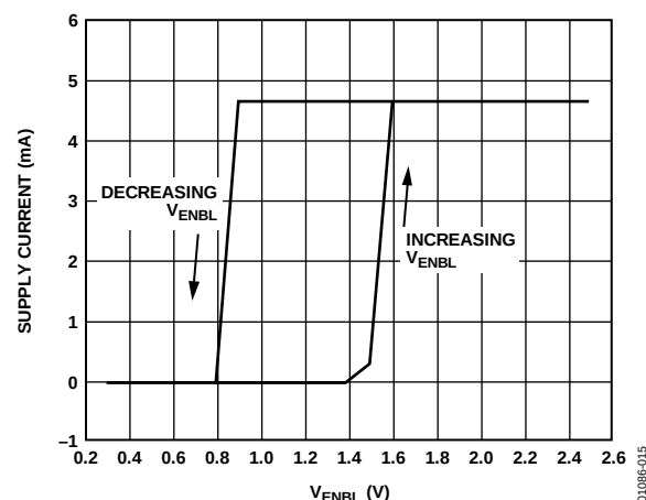
Figure 15. Supply Current vs. ENBL Voltage, V_S = 3\text{ V}
