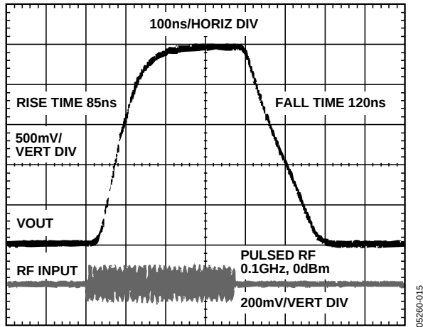
Figure 15. VOUT Response Time, RF Off to 0 dBm
