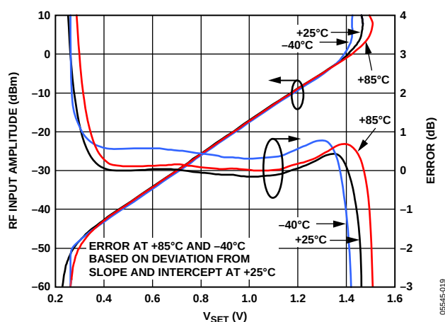
Figure 5. Input Amplitude and Log Conformance vs. V_{SET} at 0.9 GHz -40^\circ\text{C} , +25^\circ\text{C} , and +85^\circ\text{C}
