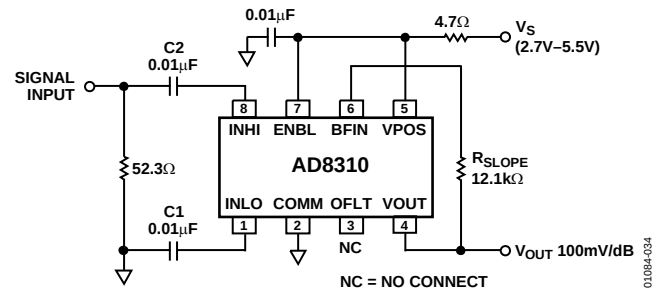
Figure 34. Raising the Slope to 100 mV/dB
