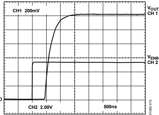
Figure 15. Power-Up Response Time
