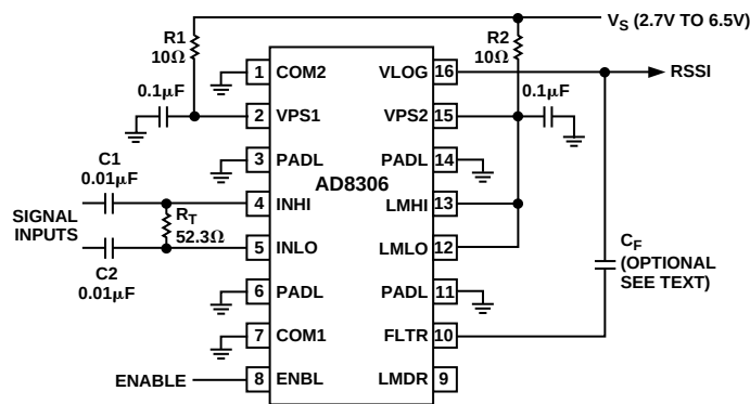
Figure 24. Basic Connections for RSSI (Log) Output
