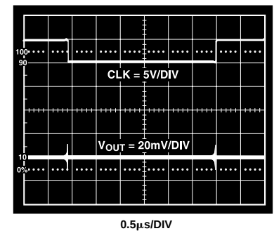
Figure 12. Digital Feedthrough vs. Time
