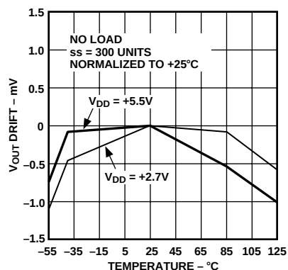
Figure 16. Full-Scale Voltage Drift vs. Temperature
