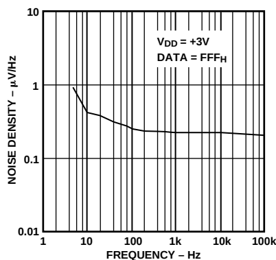
Figure 17. Output Voltage Noise Density vs. Frequency
