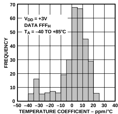
Figure 18. Full-Scale Output Tempco Histogram
