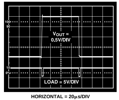
Figure 9. Large Signal Settling Time
