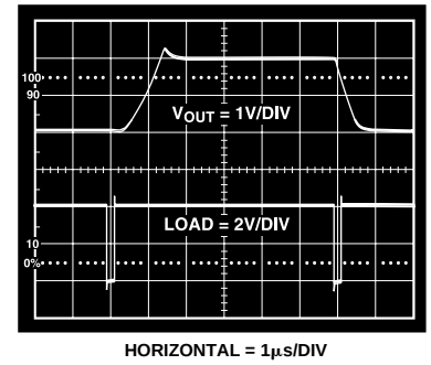
Figure 6. Detail Settling Time
