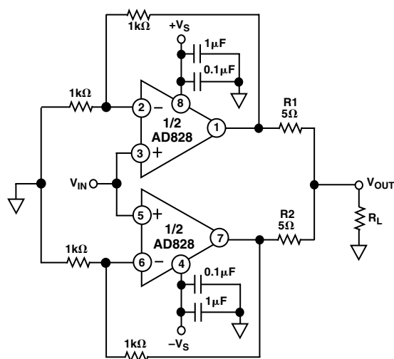
Figure 41. Parallel Amp Configuration
