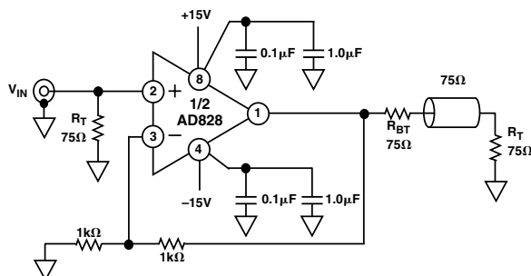
Figure 45. Video Line Driver
