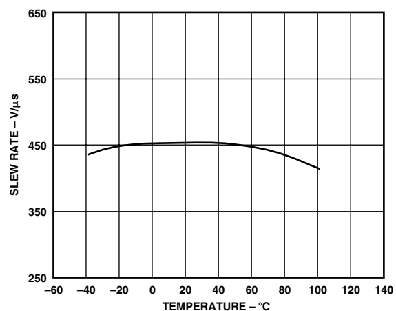
Figure 21. Slew Rate vs. Temperature
