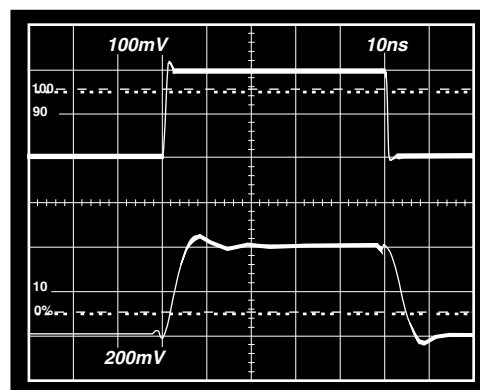
Figure 39. Noninverting Small Signal Pulse Response \pm 5 V_S , C_F = 0 \text{ pF} , R_L = 150 \Omega
