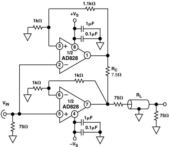
Figure 46. Low Distortion Amplifier
