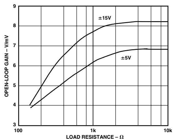
Figure 14. Open-Loop Gain vs. Load Resistance
