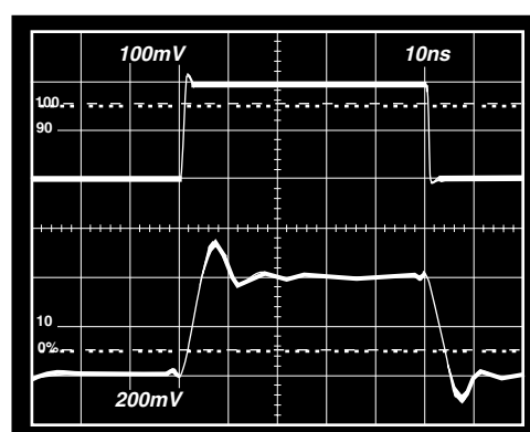
Figure 38. Noninverting Small Signal Pulse Response \pm 15 V_S , C_F = 1 \text{ pF} , R_L = 150 \Omega
