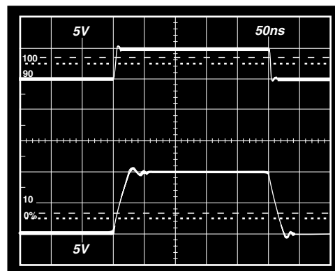
Figure 37. Noninverting Large Signal Pulse Response \pm 15 V_S , C_F = 1 \text{ pF} , R_L = 1 \text{ k}\Omega
