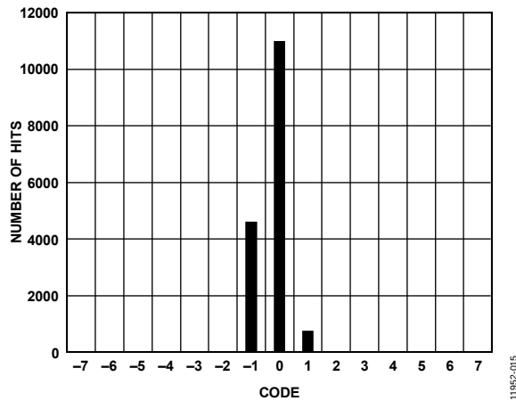
Figure 10. Output Referred Noise Histogram (Gain = 16 dB)
