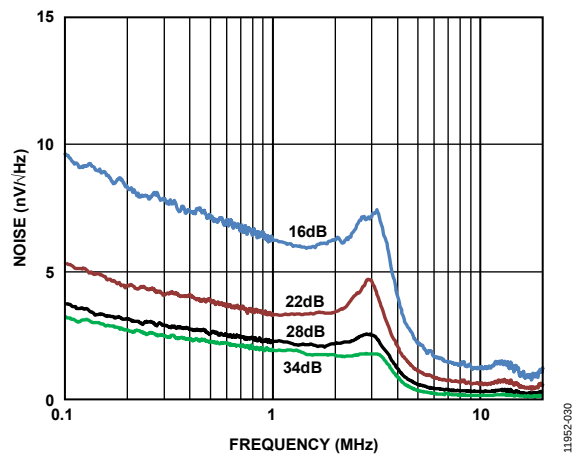
Figure 12. Short-Circuit Input Referred Noise vs. Frequency
