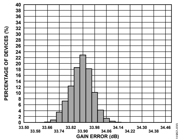
Figure 7. Gain Error Histogram (Gain = 34 dB)
