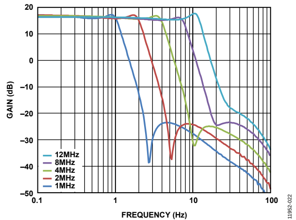
Figure 14. Filter Response
