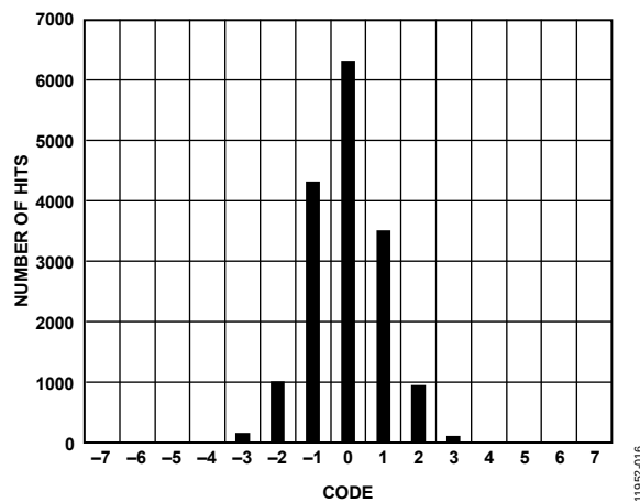
Figure 11. Output Referred Noise Histogram (Gain = 34 dB)
