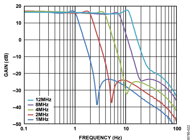
Figure 14. Filter Response
