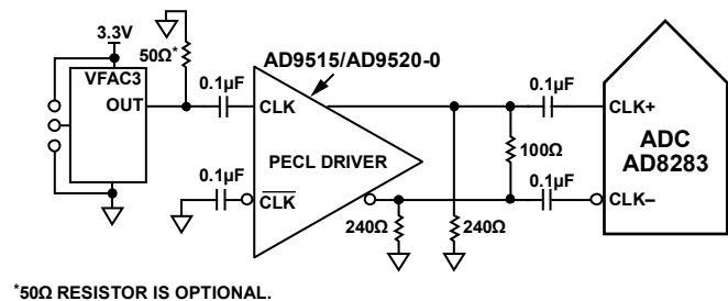
Figure 28. Differential PECL Sample Clock
