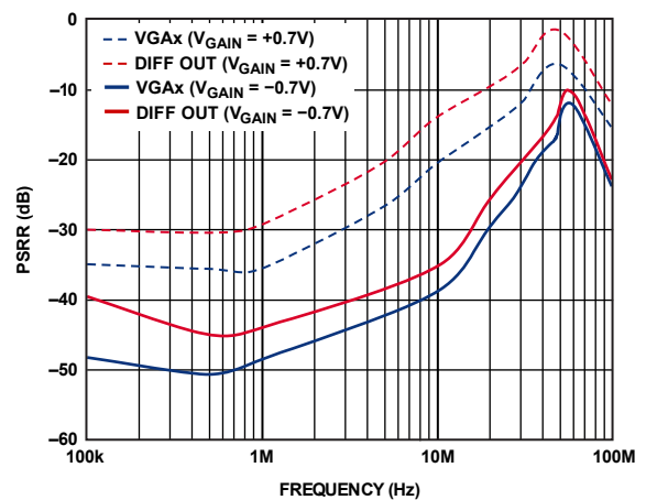
Figure 68. Power Supply Rejection vs. Frequency (VPOS)
