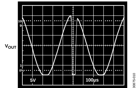
Figure 10. Phase Reversal with Inputs Exceeding Supply by 1 V
