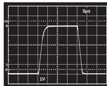
Figure 33. Pulse Response of In Amp to a 500 mV p-p Input Signal; V_s = 5\text{ V}, 0\text{ V} ; Gain = 10
