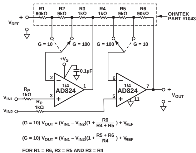
Figure 34. A Single Supply Programmable Instrumentation Amplifier
