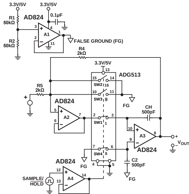
Figure 37. 3.3 V/5 V Precision Sample-and-Hold Circuit
