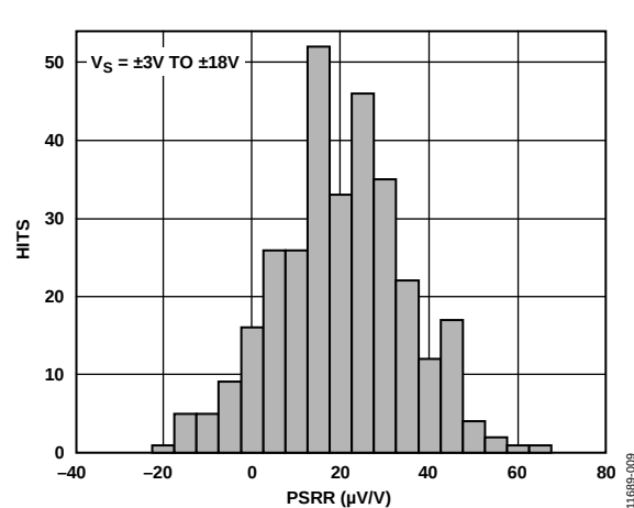
Figure 9. Typical Distribution of Power Supply Rejection Ratio (PSRR)
