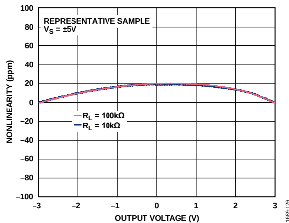
Figure 26. Nonlinearity, V_S = \pm 5V
