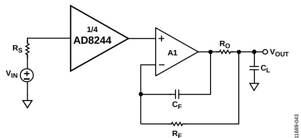
Figure 41. Adding an Op Amp for Low Output Impedance
