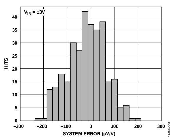
Figure 8. Typical Distribution of System Error
