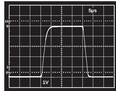
Figure 33. Pulse Response of In Amp to a 500 mV p-p Input Signal; V_s = 5V, 0V ; Gain = 10
