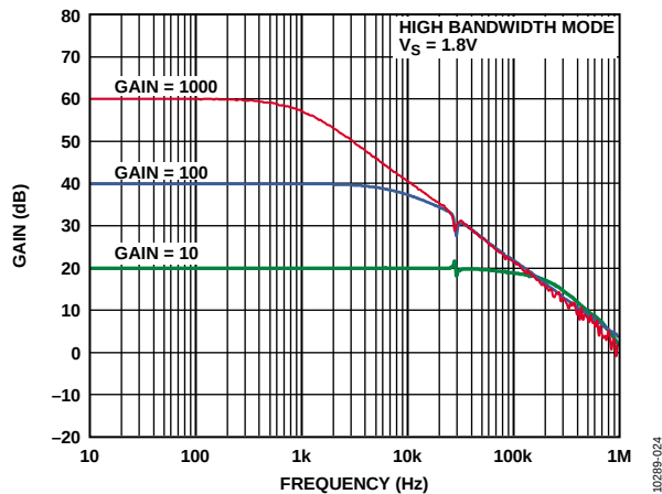
Figure 24. Gain vs. Frequency, High Bandwidth Mode, V_S = 1.8V
