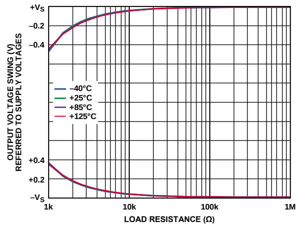
Figure 61. Output Voltage Swing vs. Load Resistance, V_S = \pm 2.5\text{ V}
