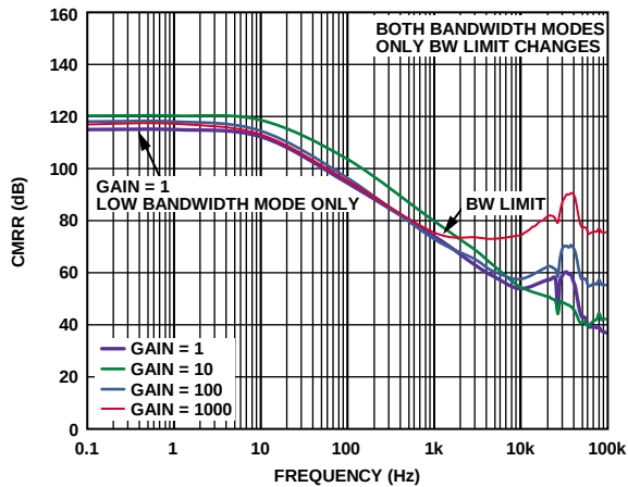
Figure 29. CMRR vs. Frequency, 1 k \Omega Source Imbalance
