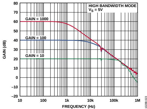
Figure 23. Gain vs. Frequency, High Bandwidth Mode, V_S = 5V
