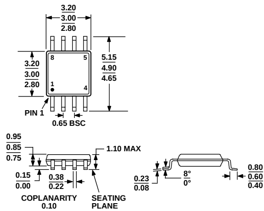
Figure 78. 8-Lead Mini Small Outline Package [MSOP] (RM-8) Dimensions shown in millimeters
