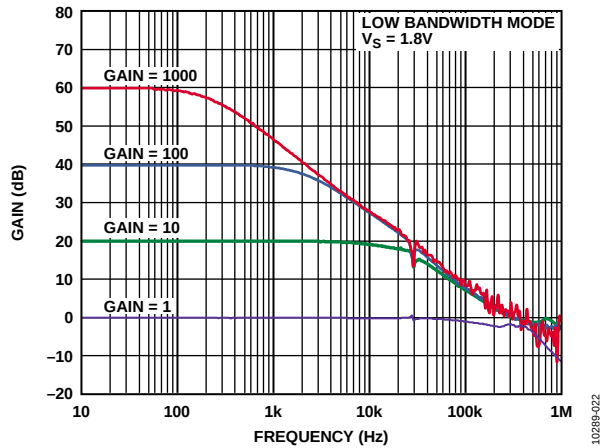
Figure 22. Gain vs. Frequency, Low Bandwidth Mode, V_S = 1.8V
