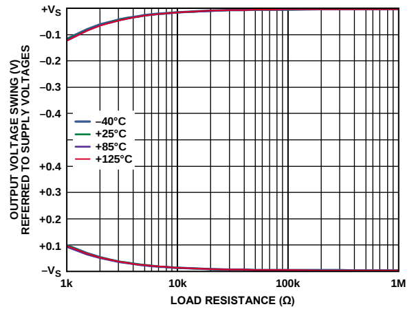
Figure 62. Output Voltage Swing vs. Load Resistance, V_S = \pm 0.9\text{ V}
