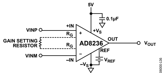
Figure 35. Basic Setup
