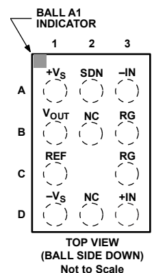
Figure 2. 11-Ball WLCSP (CB-11-1)
