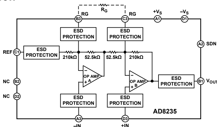
Figure 35. Simplified Schematic
