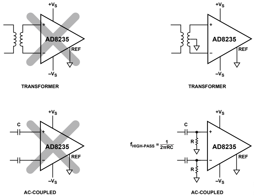
Figure 40. Creating an I_{BIAS} Path
