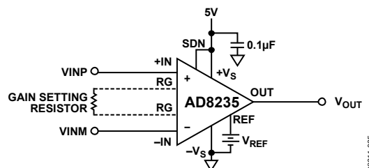
Figure 36. Basic Setup
