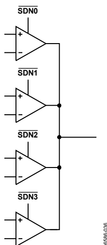
Figure 54. Four AD8231s in Multiplexing Configuration
