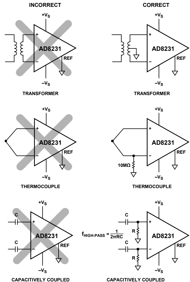
Figure 51. Creating an I_{BIAS} Path
