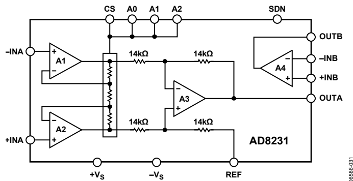
Figure 49. Simplified Schematic
