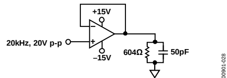
Figure 28. Output Swing, V_S = \pm 15\text{ V} , G = +1
