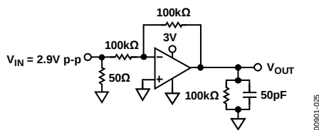
Figure 25. Output Swing, +V_S = +3\text{ V} , G = -1
