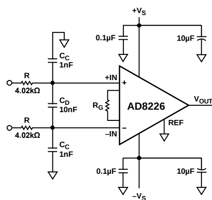
Figure 8. RFI Suppression
