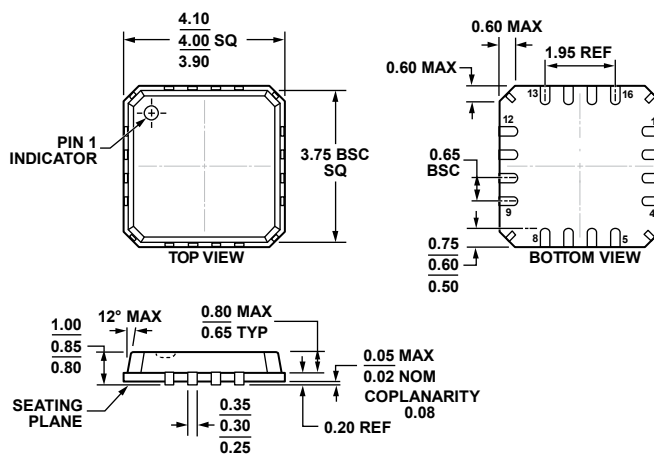
Figure 56. 16-Lead Lead Frame Chip Scale Package [LFCSP] 4 mm × 4 mm Body and 0.85 mm Package Height with Hidden Paddle (CP-16-19)
