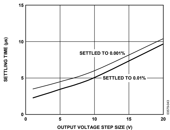
Figure 53. Settling Time vs. Output Voltage Step Size ( G = 1 ) \pm 15\text{ V} , V_{\text{REF}} = 0\text{ V}
