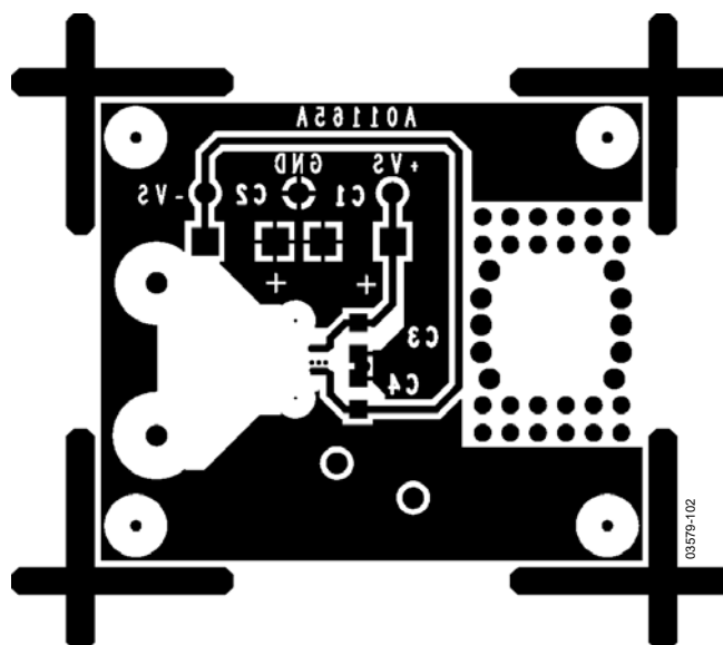
Figure 58. Example Layout—Bottom Layer of the AD8220 Evaluation Board
