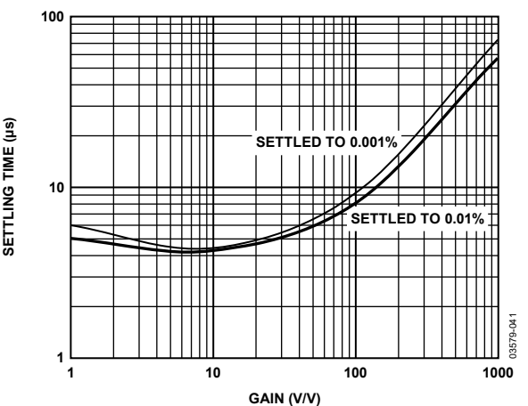
Figure 54. Settling Time vs. Gain for a 10 V Step, V_s = \pm 15\text{ V} , V_{\text{REF}} = 0\text{ V}
