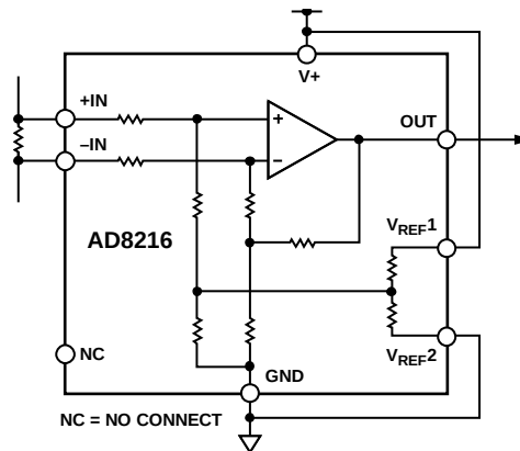
Figure 27. Split Supply
