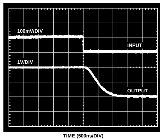
Figure 13. Fall Time
