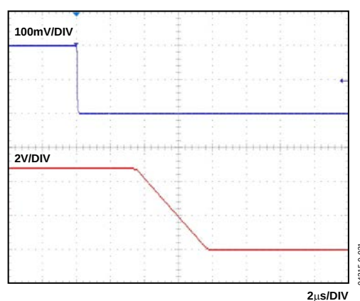
Figure 9. Differential Overload Recovery (Falling)
