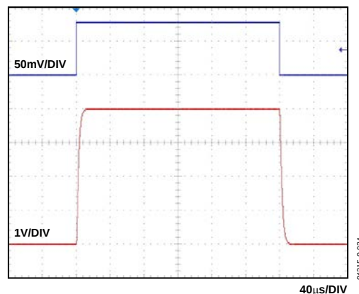
Figure 8. Rise/Fall Time
