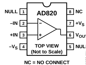
Figure 1. 8-Lead PDIP
