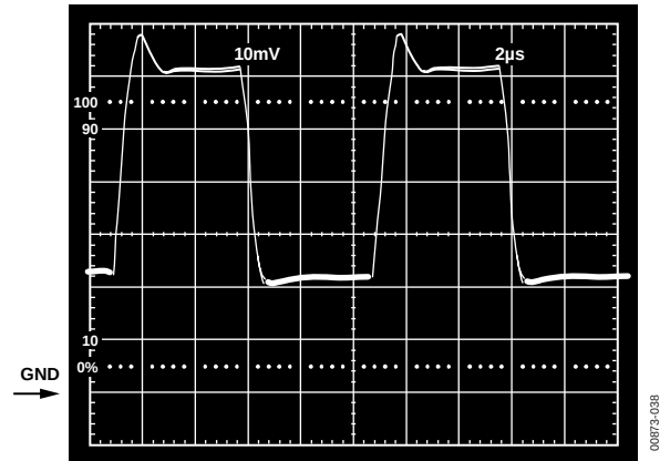
Figure 37. V_S = 5\text{ V} , 0\text{ V} ; Gain-of-2 Inverter Response to 20\text{ mV} Step, Centered 20\text{ mV} Below Ground
