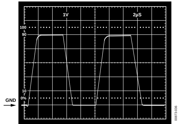
Figure 36. V_S = 5\text{ V} , 0\text{ V} ; Gain-of-2 Inverter Response to 2.5\text{ V} Step, Centered -1.25\text{ V} Below Ground
