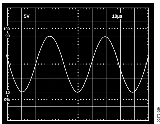
Figure 28. 20 V, 25 kHz Sine Input; Unity-Gain Follower; R_L = 600\ \Omega , V_S = \pm 15\text{ V}
