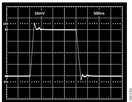
Figure 31. Small Signal Response Unity-Gain Follower; V_S = \pm 15\text{ V} , R_L = 10\text{ k}\Omega
