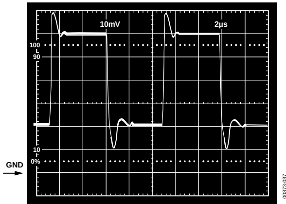
Figure 34. V_S = 5\text{ V} , 0\text{ V} ; Unity-Gain Follower Response to 40\text{ mV} Step Centered 40\text{ mV} Above Ground
