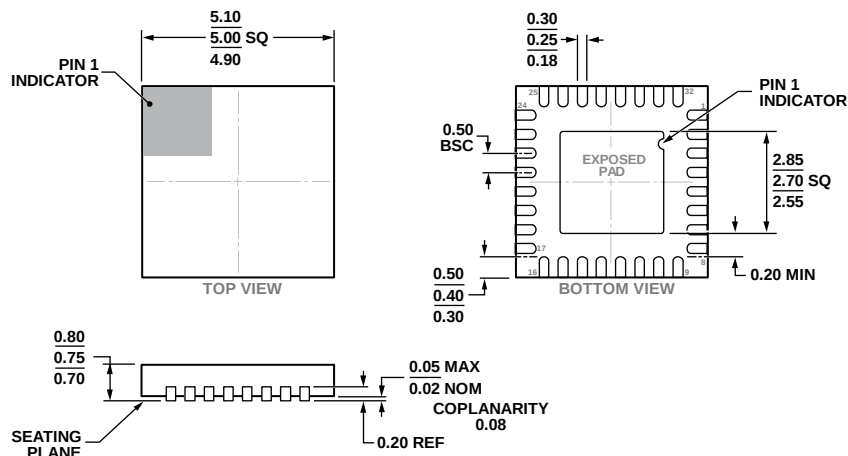
Figure 27. 32-Lead Lead Frame Chip Scale Package [LFCSP] 5 mm × 5 mm Body and 0.75 mm Package Height (CP-32-21)
