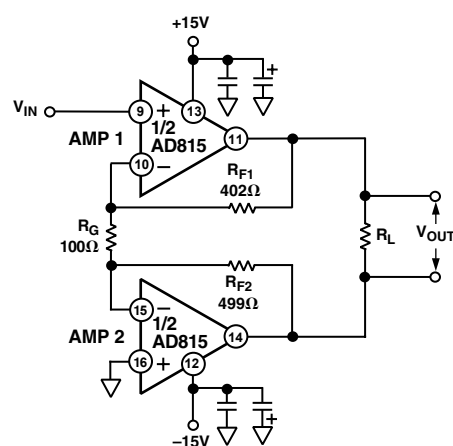
Figure 54. Direct Single-Ended-to-Differential Conversion
