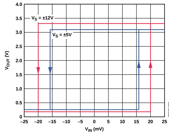
Figure 36. Comparator Hysteresis
