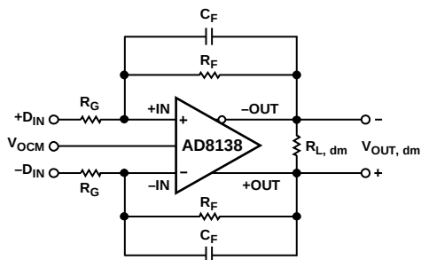
Figure 42. Circuit Definitions
