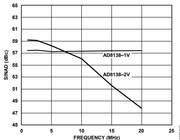
Figure 49. AD9203 SINAD at -0.5 dBFS AD8138
