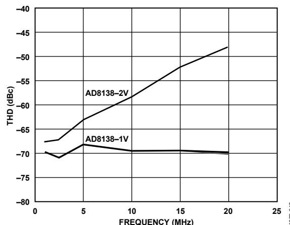
Figure 48. AD9203 THD at -0.5 dBFS AD8138
