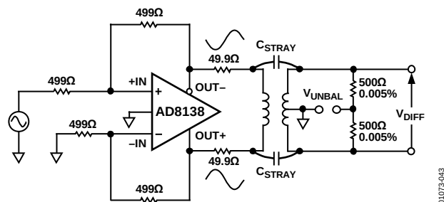
Figure 44. AD8138 Forms a Balanced Transformer Driver
