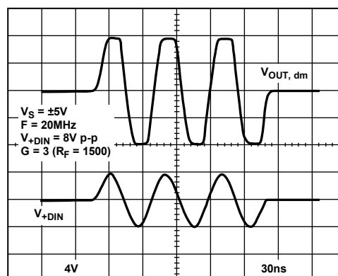
Figure 26. Output Overdrive
