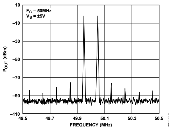
Figure 19. Intermodulation Distortion
