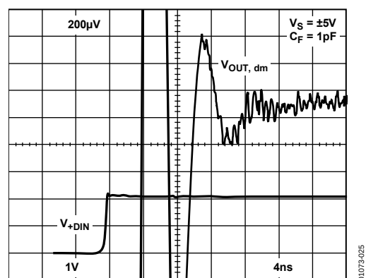
Figure 25. Settling Time
