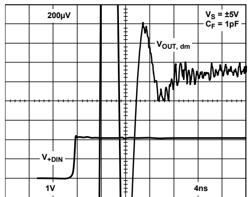
Figure 25. Settling Time
