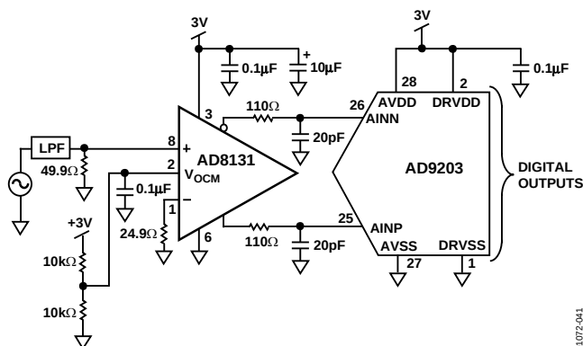
Figure 41. Test Circuit for AD8131 Driving an AD9203, 10-Bit, 40 MSPS ADC
