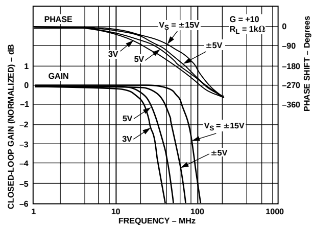
Figure 32. Closed-Loop Gain and Phase vs. Frequency, Gain = +10, R_L = 1\ \text{k}\Omega
