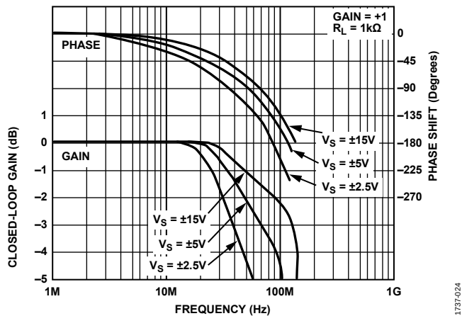
Figure 26. Closed-Loop Gain and Phase Shift vs. Frequency, G = +1 , R_F = 1 \text{ k}\Omega for \pm 15 \text{ V} , 910 \Omega for \pm 5 \text{ V} and \pm 2.5 \text{ V}
