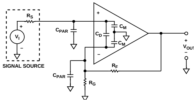
Figure 43. Input and Board Capacitances
