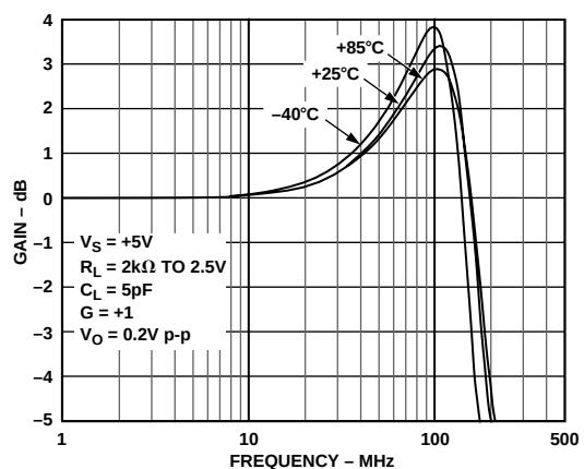
Figure 8. AD8054 Gain vs. Frequency vs. Temperature
