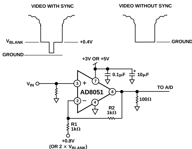
Figure 47. Sync Stripper
