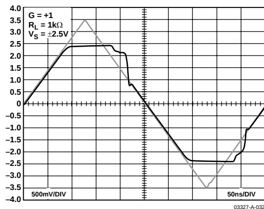
图33. 输入过驱恢复
