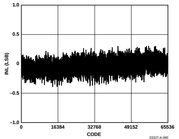
图61. 积分非线性
