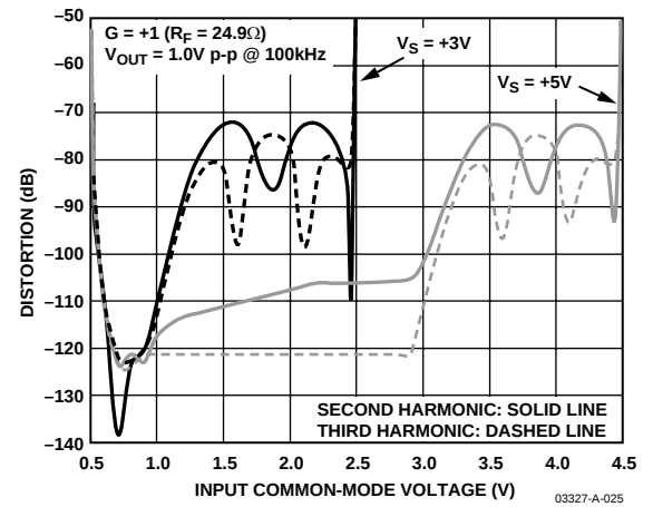
Figure 26. Harmonic Distortion vs. Input Common-Mode Voltage, SELECT = Three\text{-}State\text{ or }Open
