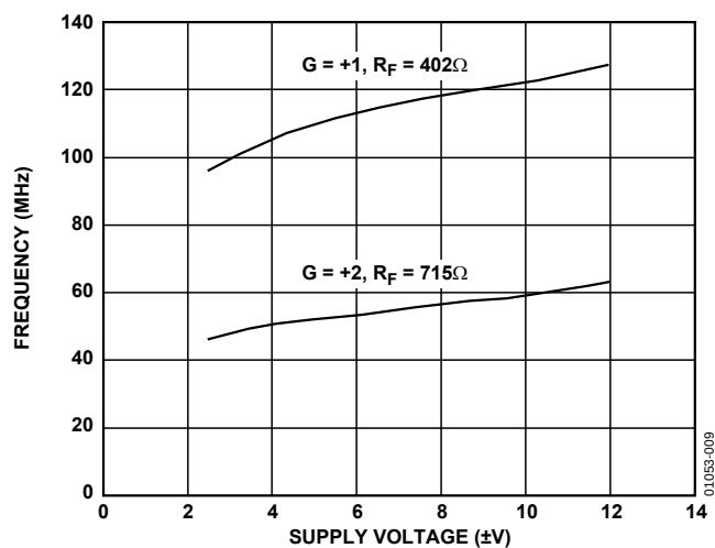
Figure 9. Bandwidth vs. Supply, R_L = 500\Omega , V_{IN} = 200\text{ mV p-p}
