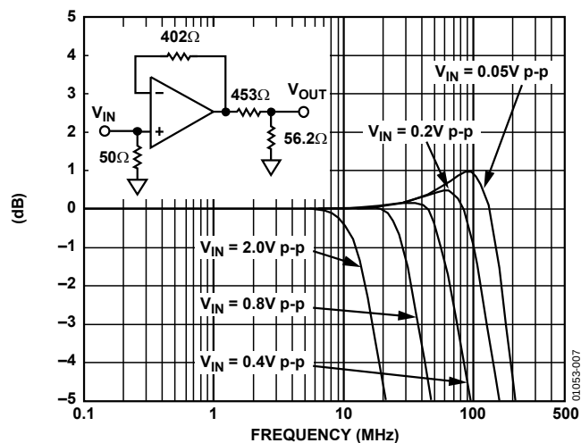
Figure 7. Frequency Response vs. Signal Level, V_S = \pm 12\text{ V} , G = +1
