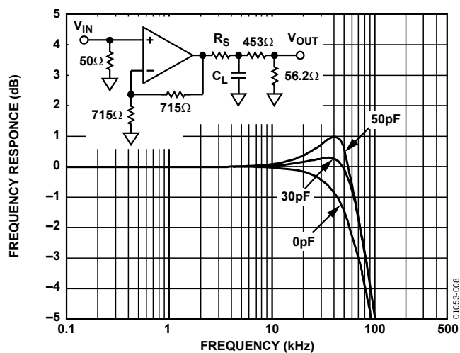
Figure 8. Frequency Response vs. Capacitive Load; C_L = 0\text{ pF} and 50\text{ pF} ; R_S = 0\Omega
