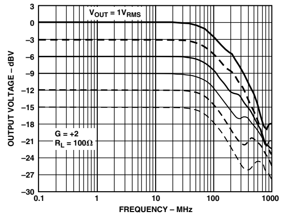
TPC 22. Output Voltage vs. Frequency; V_S = \pm 2.5\text{ V}
