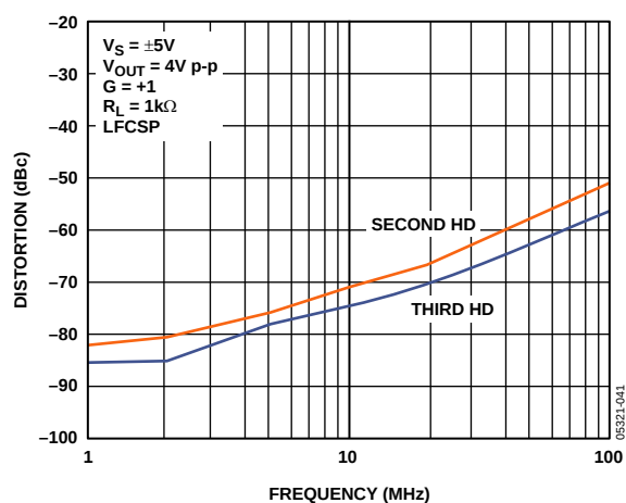
Figure 21. Harmonic Distortion vs. Frequency
