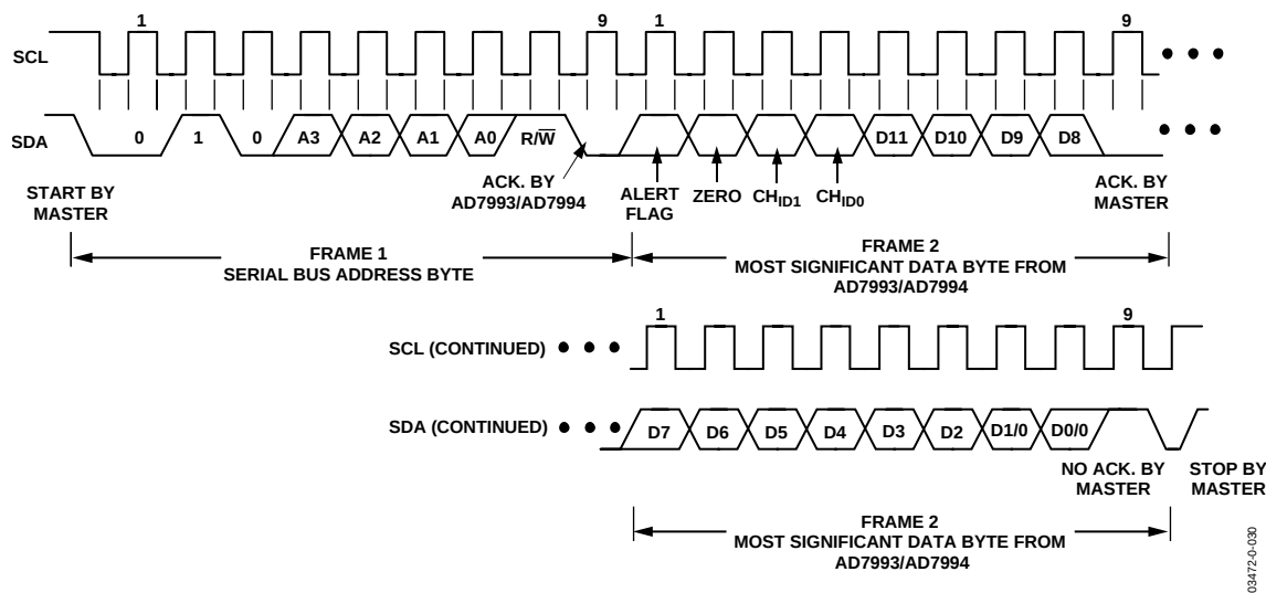
Figure 30. Reading Two Bytes of Data from the Conversion Result Register
