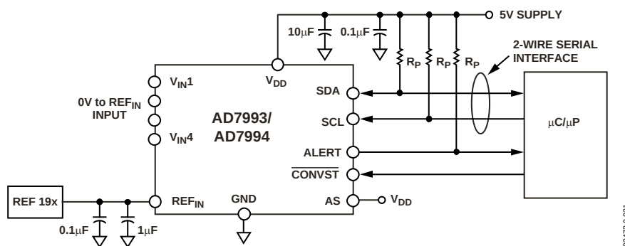
Figure 22. AD7993/AD7994 Typical Connection Diagram
