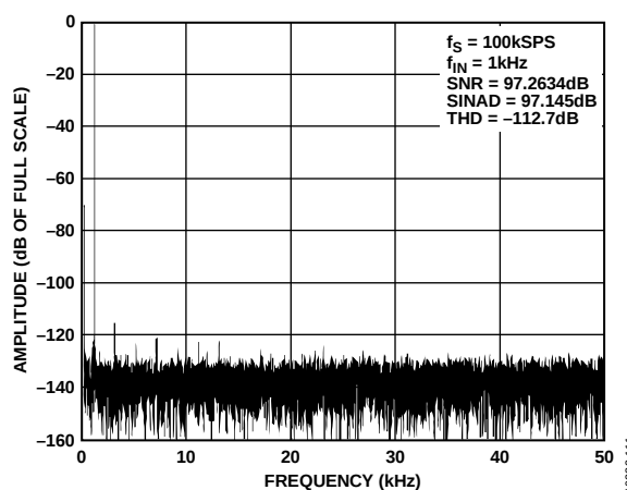
Figure 10. AD7989-1 FFT Plot
