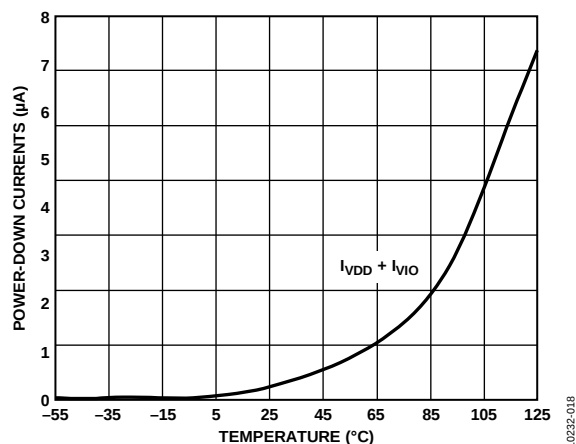
Figure 21. Power-Down Currents vs. Temperature
