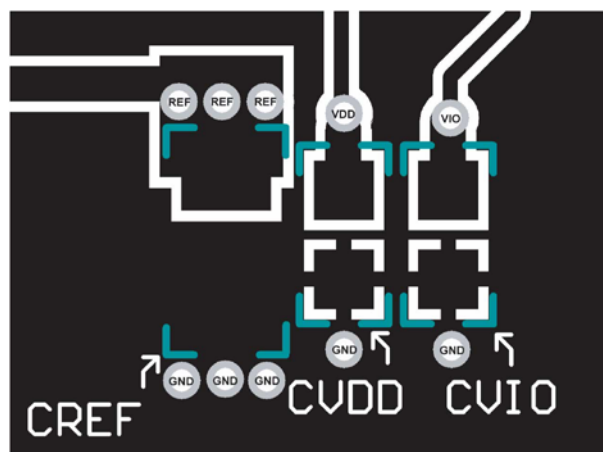
Figure 39. Recommended Layout of the AD7989-1/AD7989-5 (Bottom Layer)
