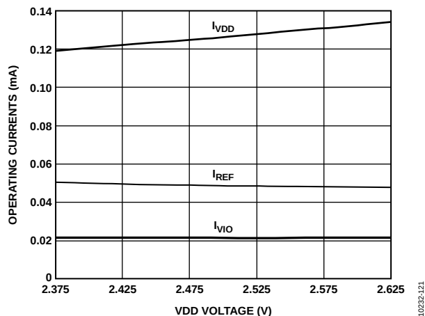
Figure 20. Operating Currents vs. VDD Voltage (AD7989-1)
