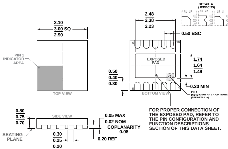
Figure 44. 10-Lead Lead Frame Chip Scale Package [LFCSP] 3 mm x 3 mm Body and 0.75 mm Package Height (CP-10-9)
