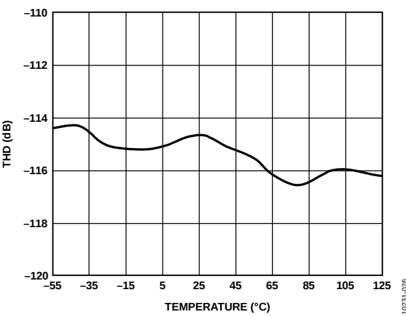
Figure 24. THD vs. Temperature
